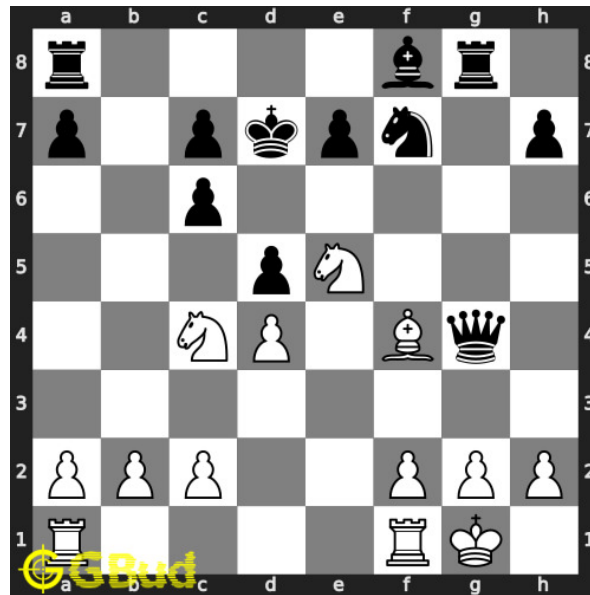
Figure 10: Nfe5+ - You can fork the opponent's king and queen using the knight from e5, but e5 is guarded by their knight. One of your knights is sacrificing itself to gain the queen
