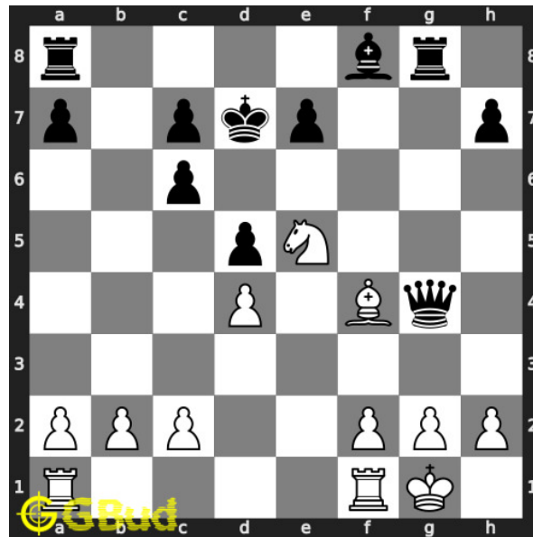
Figure 6: Nxe5+ - Your next knight captures the opponent's knight and forks king and queen. Now the king is forced to move.
