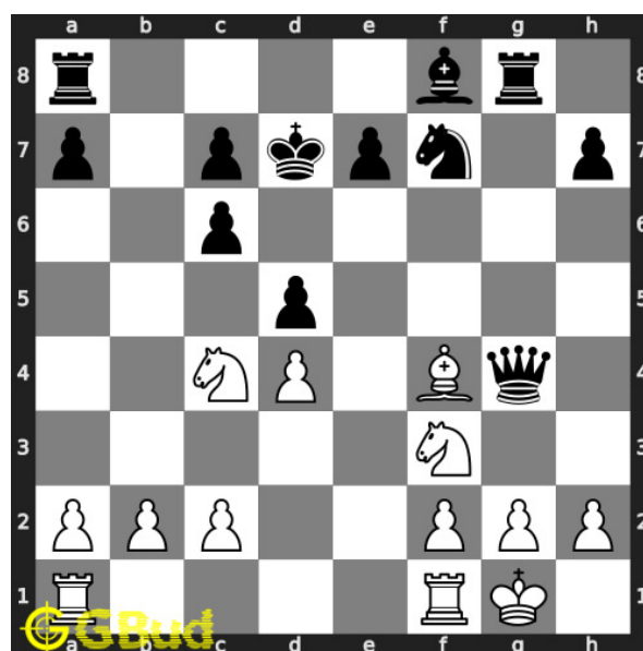
Figure 9: Initial board position of medium chess puzzle 0079
