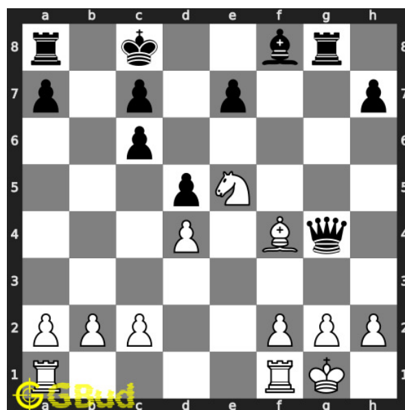
Figure 13: Kc8 - Since there are no pieces to capture your knight, king moves to c8 to escape from the check threat
