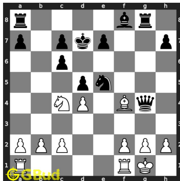
Figure 11: Nxe5 - Opponent's knight captures yours
