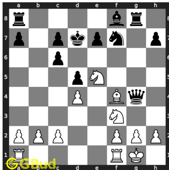
Figure 4: Nce5+ - You can fork the opponent's king and queen using the knight from e5, but e5 is guarded by their knight. One of your knights is sacrificing itself to gain the queen
