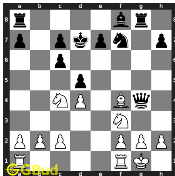
Figure 1: Solve this medium chess puzzle 0079. Gain queen in three moves @ https://gbud.in/gs34f32
